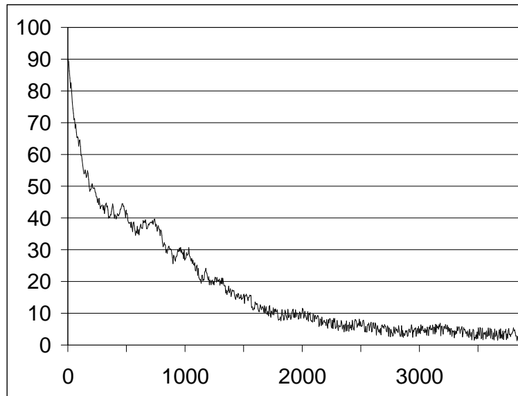
Figure 4: The percentage of agents in the population which can not “decide” which types of agents they should trust. In the beginning of the run, this percentage is high as most agents change their preference in every time step, more or less randomly guessing. After a while, fixed preferences evolve.
