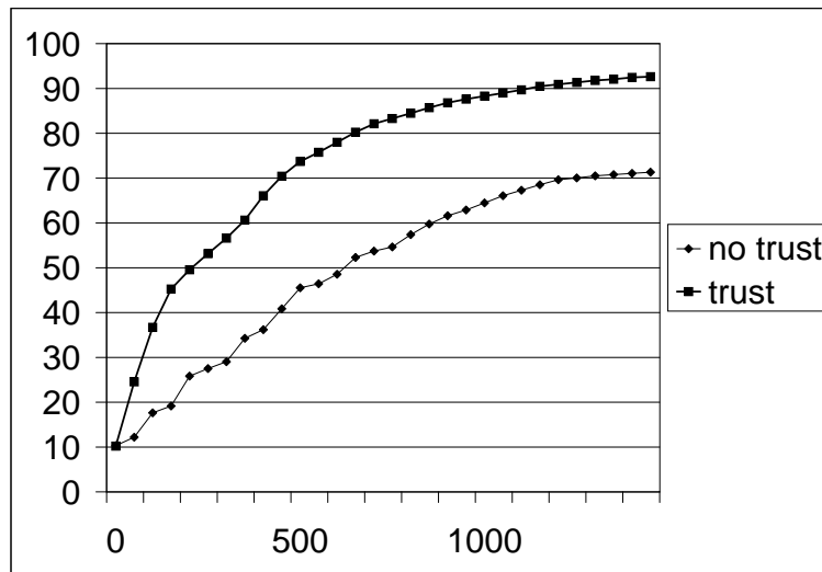
Figure 5: The general cooperation levels, averaged from respectively fifty runs with and without a co-evolution of trust. When trust is activated, a higher general cooperation level is reached much faster than without trust.
